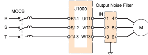
Connection Diagram
